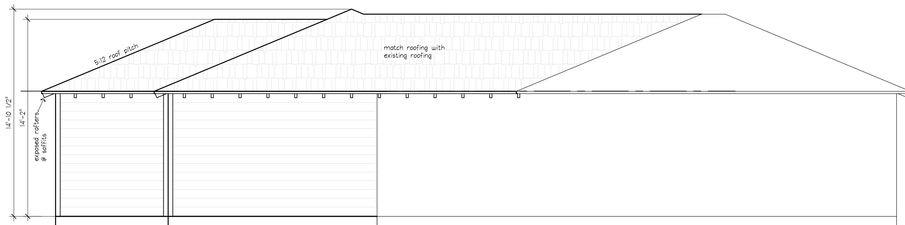
LEFT ELEVATION
